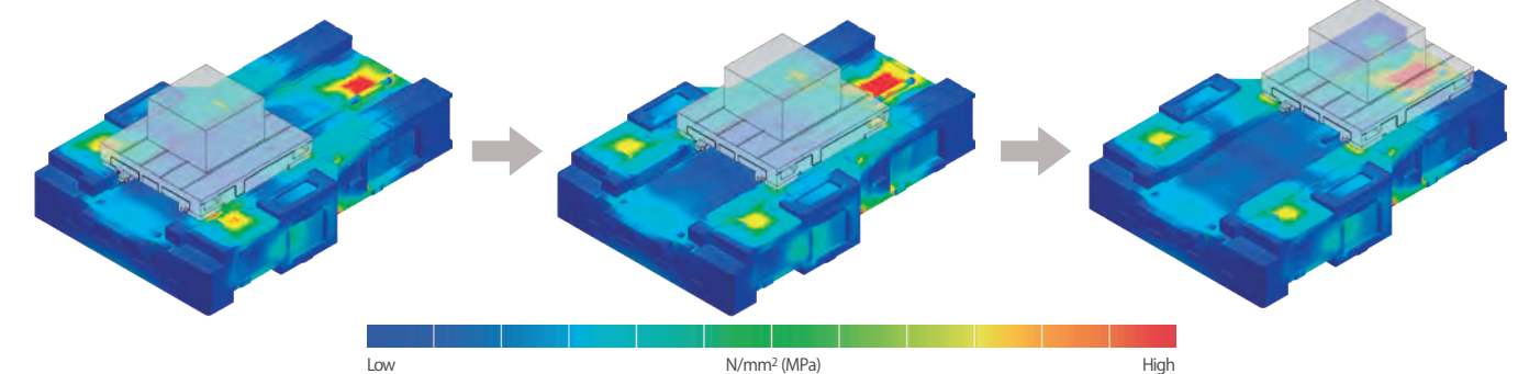
FEM structural analysis simulation
