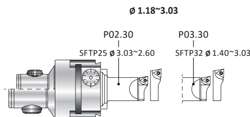
Working Range
