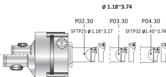
Working Range
